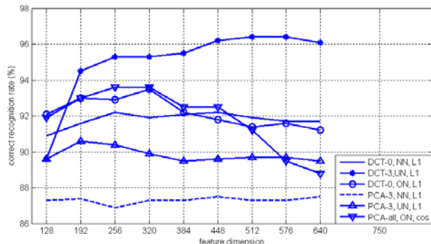
Figure 6. Correct recognition rate vs. feature dimension plot for feature selection, feature normalization and distance metric combinations
