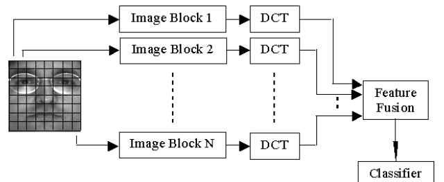
Figure 3. The diagram of feature extraction
