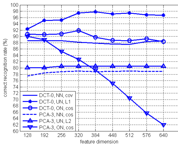
Figure 8. Correct recognition rate vs. feature dimension plot for feature selection, feature normalization and distance metric combinations
