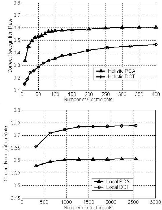
Figure 5: Correct recognition rate versus number of used coefficients on the CMU PIE database. First row: Holistic PCA vs. holistic DCT. Second row: Local PCA vs. local DCT.
