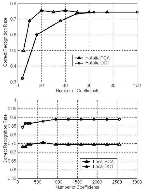
Figure 3: Correct recognition rate versus number of used coefficients on the Yale database. First row: Holistic PCA vs. holistic DCT. Second row: Local PCA vs. local DCT.
